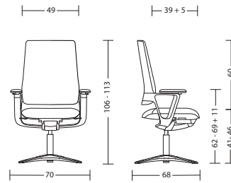
cnx90 + 3314 with arm supports: cnx90 - 20 kg
