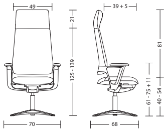
cnx91 + 3314 with arm supports: cnx91 - 22 kg
