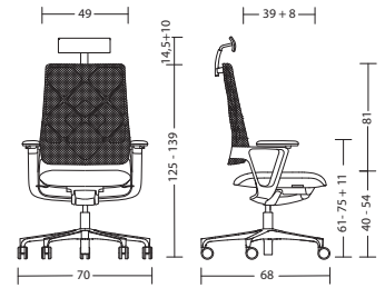
cnx89 with arm supports: cnx89 - 20 kg
