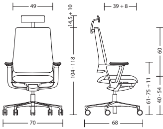
cnx99 with arm supports: cnx99 - 20 kg
