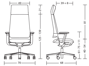
cnx95 with arm supports: cnx95 - 22 kg
