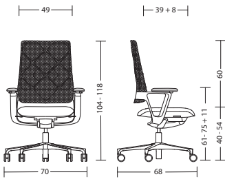
cnx88 with arm supports: cnx88 - 18 kg
