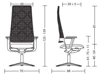
cnx81 + 3314 with arm supports: cnx81 - 22 kg
